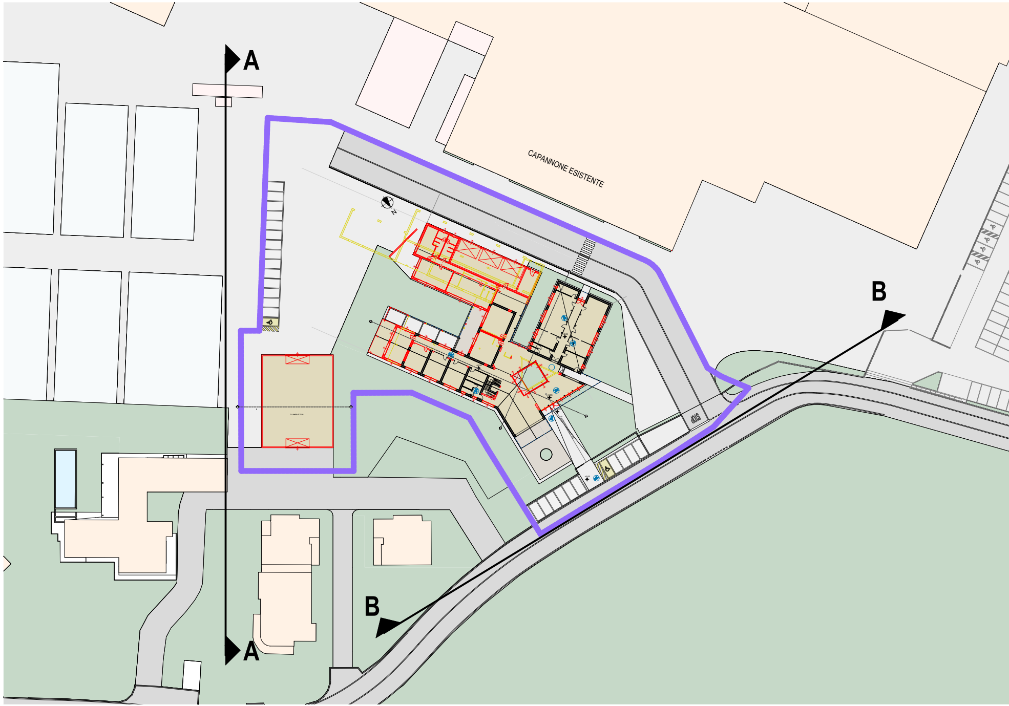
KEYPLAN - SCALA 1:1000
